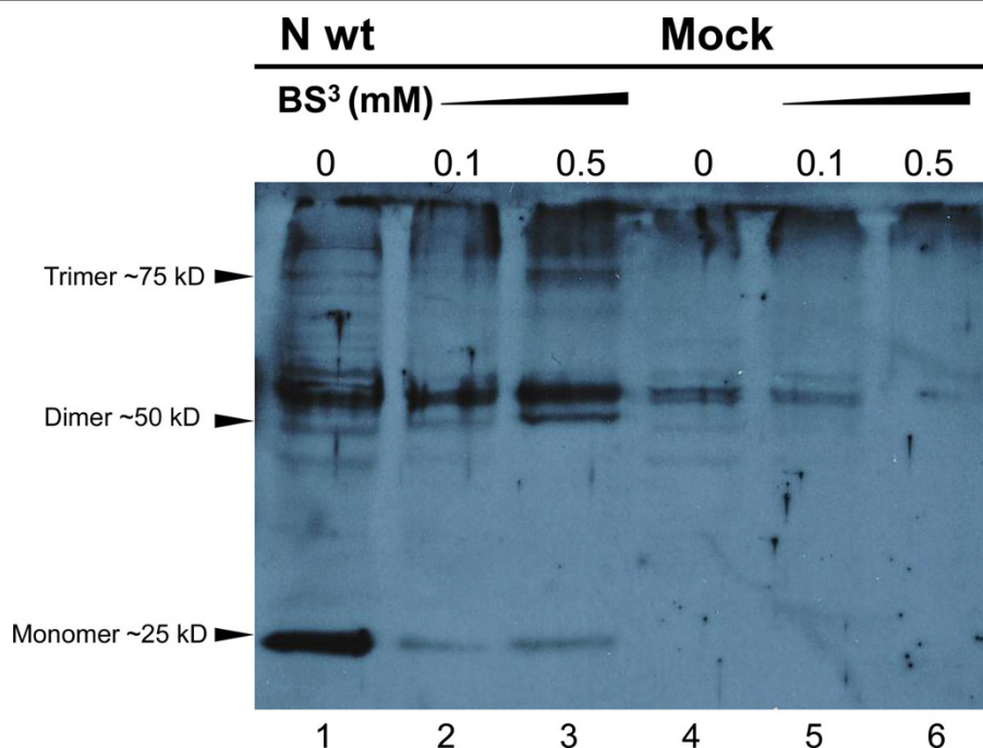
Figure 1 Cross-linking of the UUKV-N protein. N protein containing COS-7 cell lysates were treated with 0.1 or 0.5 mM of cross-linking reagent (BS 3 ), and resolved by 10% SDS-PAGE under denaturing conditions. An immunoblot shows that omitting BS 3 , the majority of the full-length UUKV-N protein migrated as 25 kDa monomeric form (lane 1). Addition of BS 3 decreased the amount of the monomeric form, while the amount of dimeric and multimeric forms were simultaneously increasing (lanes 2 and 3). In mock-transfected samples no N protein was detected (lanes 4 to 6).
